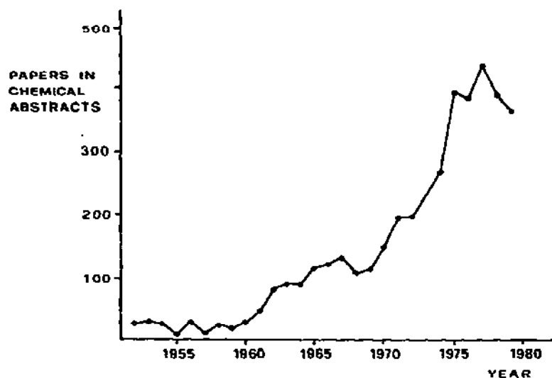
Fig. 1. Number of technetium studies reported in Chemical Abstracts as a function of year.
