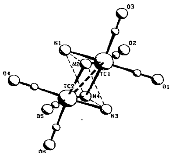
Fig. 20. \text{TPP}[\text{Tc}(\text{CO})_3]_2 .
