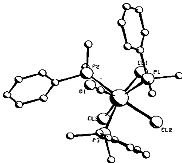
Fig. 16. \text{TcCl}_3(\text{CO})(\text{PMe}_2\text{Ph})_3 .
