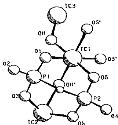
Fig. 26. A portion of the [\text{Tc}(\text{OH})(\text{MDP})]_n^- polymeric structure.
