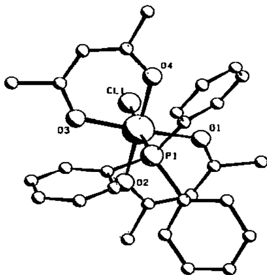
Fig. 17. tr - \text{Tc}(\text{acac})_2(\text{PPh}_3)\text{Cl} .
