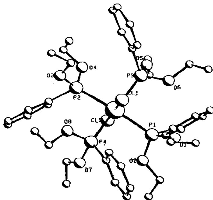
Fig. 18. tr\text{-Tc}(\text{PPh}(\text{OEt})_2)_4\text{Cl}_2 .
