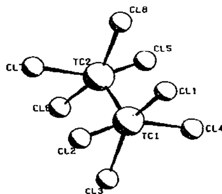
Fig. 9. [\text{Tc}_2\text{Cl}_8]^{3-} .
