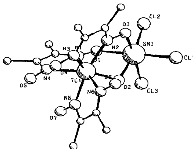
Fig. 27. \text{Tc}(\text{dmgl})_3(\text{SnCl}_3)(\text{OH}) .
